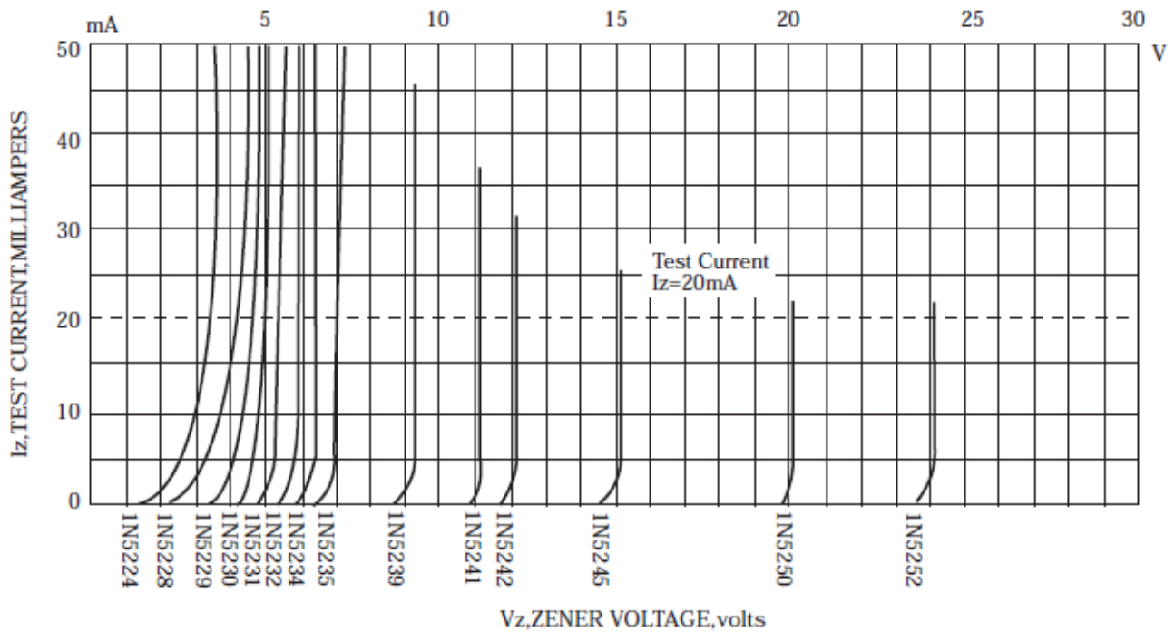
Fig.1 Breakdown Characteristics
